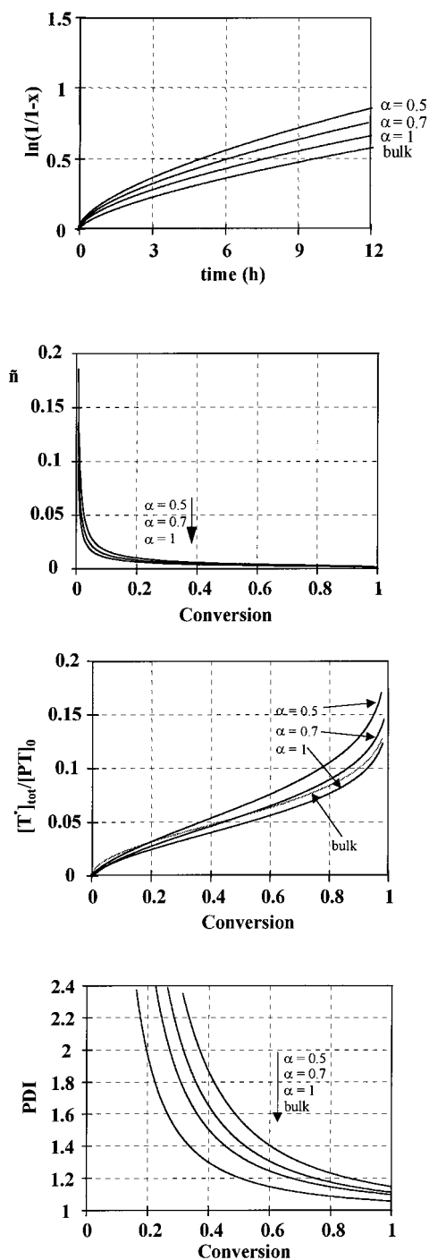
Figure 3. SG1-mediated CRP of styrene at 90 °C. Effect of \alpha when [P-T]_0 = 0.05 \text{ mol} \cdot \text{L}^{-1} , [T^*]_0 = 0 , and D = 100 \text{ nm} .
